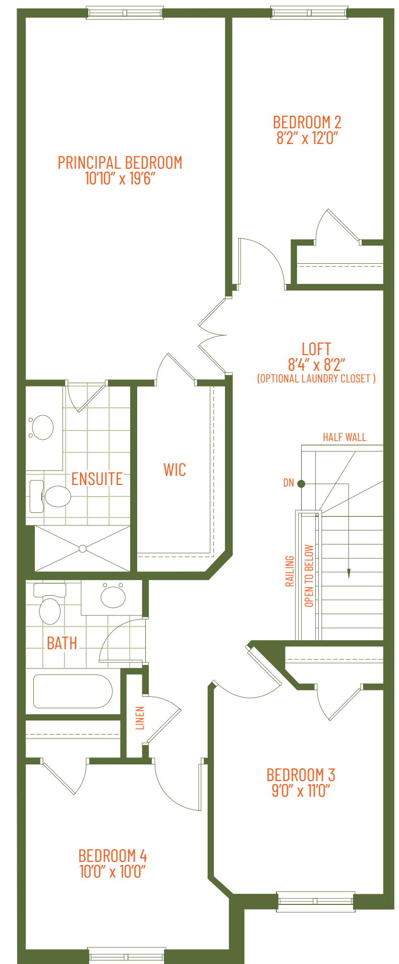
OPTIONAL INTERIOR 4 BEDROOM SECOND FLOOR PLAN
